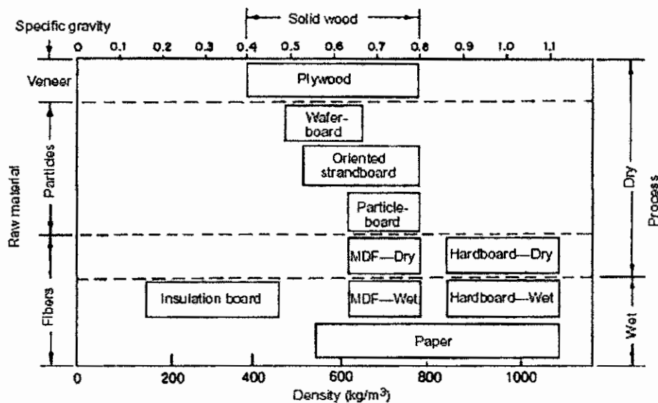
Figure-9: Classification of wood composite boards by particle size, density and process type (Suchsland and Woodson, 1986).
